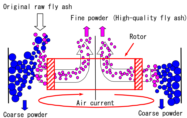
Figure 1. Schematic diagram of centrifugal machine in production of classified fine fly ash
