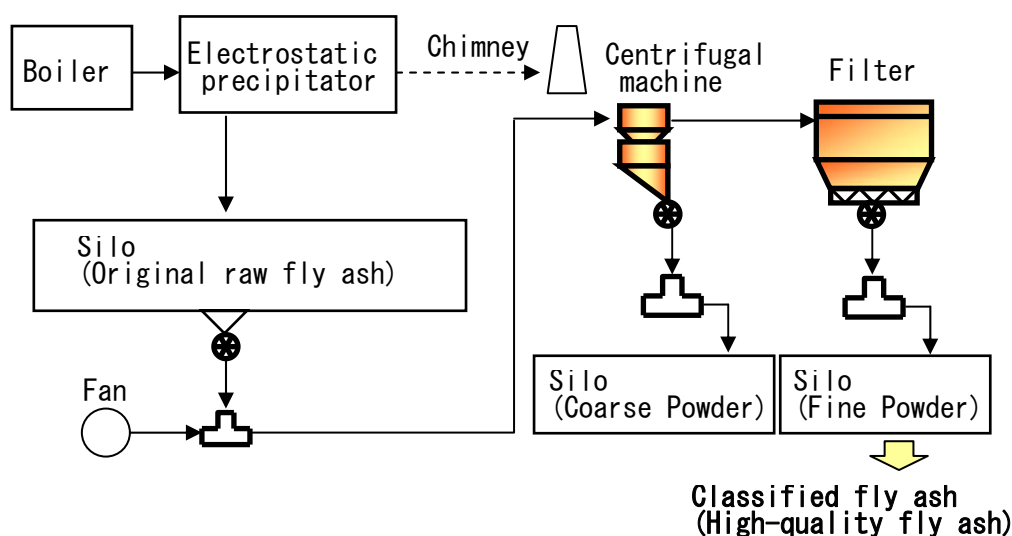
Figure 4. Production process of classified fly ash in Nanao-Ohta coal burning power plant in Ishikawa Prefecture
