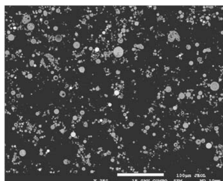
Photograph 2. Size and shape of classified fly ash particles (Scale:100 μ m)
