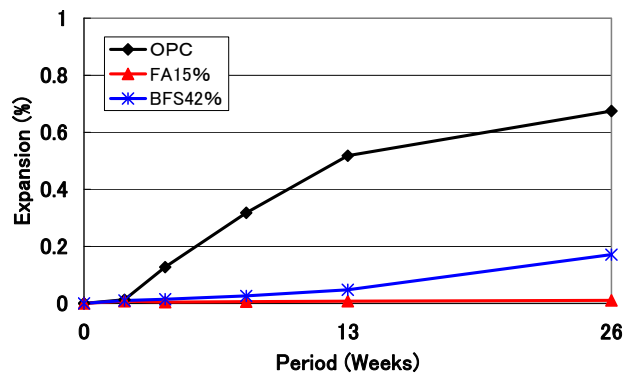
Figure 5. Expansion behaviors of OPC, BFS 42% and FA 15 % mortars in JIS A1146 method
