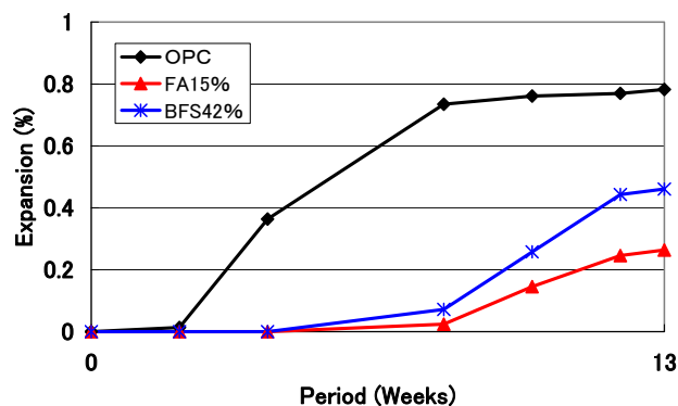
Figure 6. Expansion behaviors of OPC, BFS 42% and FA 15 % mortars in Danish method
