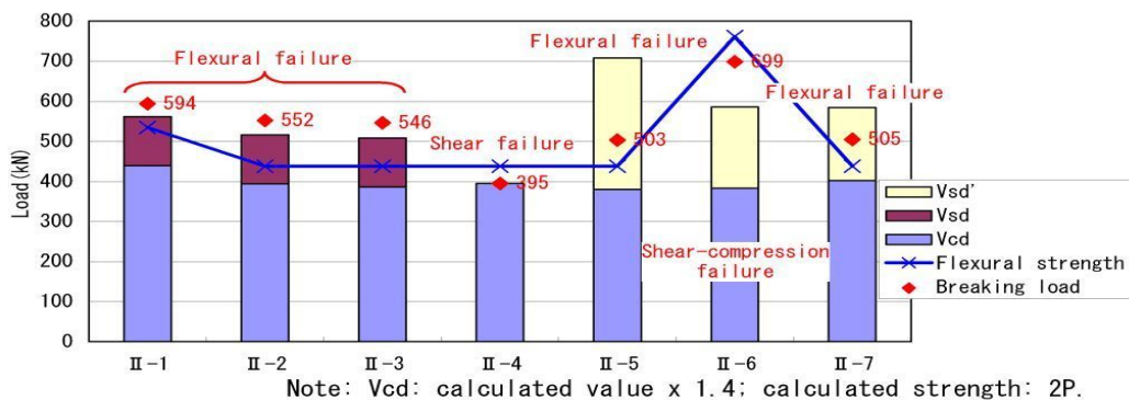
Figure 6. Calculated strengths and actual breaking loads
