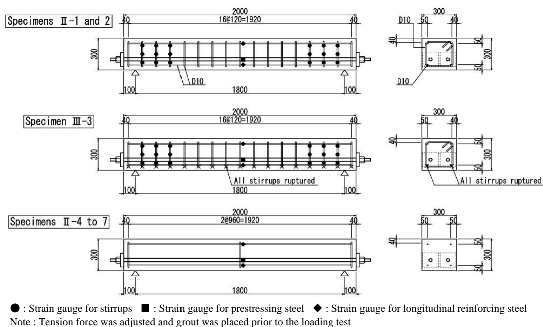
Figure 1. Structural diagrams of the specimens
