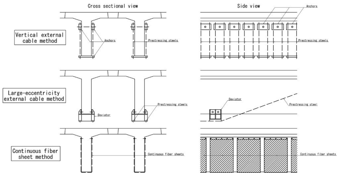
Figure 2. Schematic views of the strengthening methods
