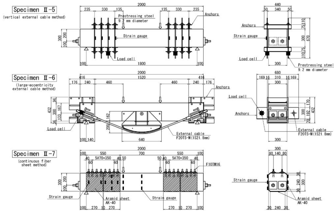
Figure 3. Structural diagrams of the strengthened specimens
