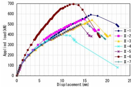
Figure 7. Load-displacement curves
