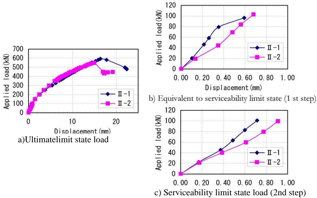
Figure 8. Load-displacement curves (II-1 and 2)
