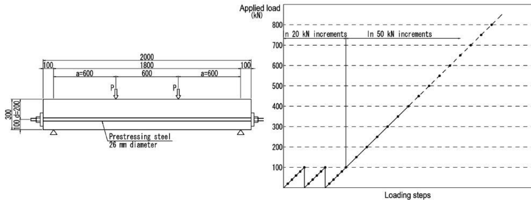
Figure 5. Loading positions and steps
