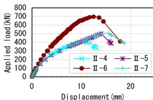
Figure 10. Load-displacement curves (II-4 to 7)
