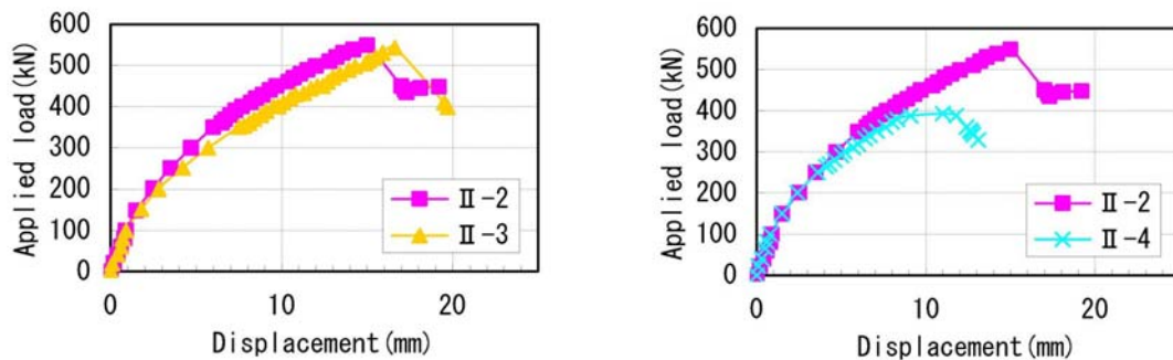
Figure 9. Load-displacement curves (II-2 to 4)
