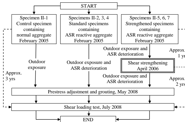
Figure 4. Flow of the experiment
