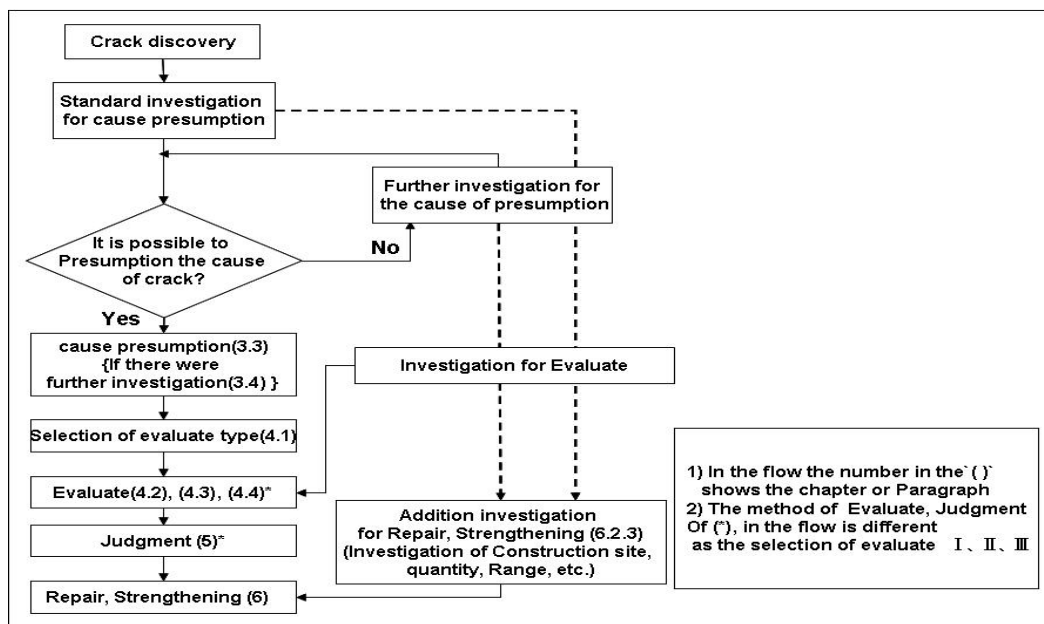
Figure1. Procedure from the investigation of cracks to the application of repair and strengthening
