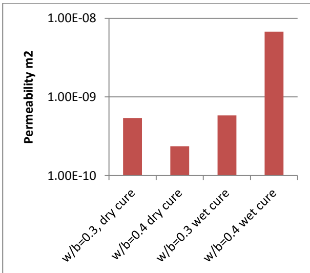
Figure 5 28 Day permeability for mixes with 2.5% SP, 42.5% IFA, 10% SF, 15% BPD, 30% GGBS
