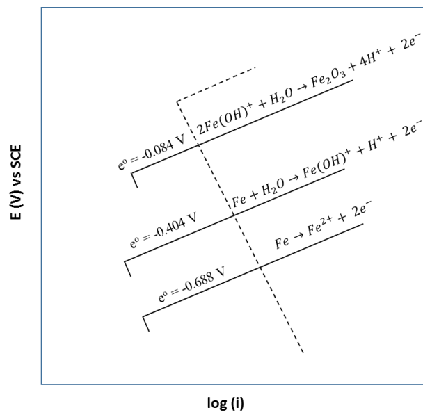
Fig. 2 Corrosion reaction mechanism adopted from [1]
