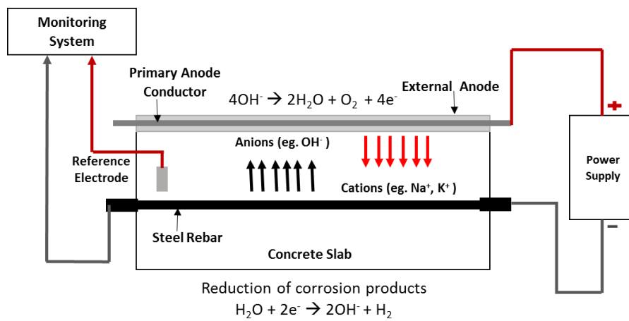
Fig. 10 Schematic of Electrochemical Realkalization
