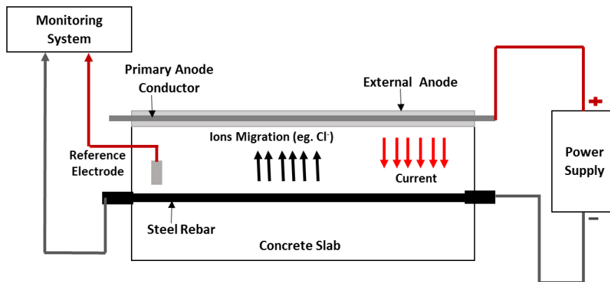
Fig. 9 Schematic of Impressed Current Cathodic Protection System
