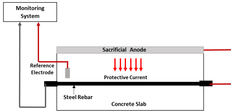
Fig. 8 Schematic of Sacrificial Anodic Cathodic Protection System
