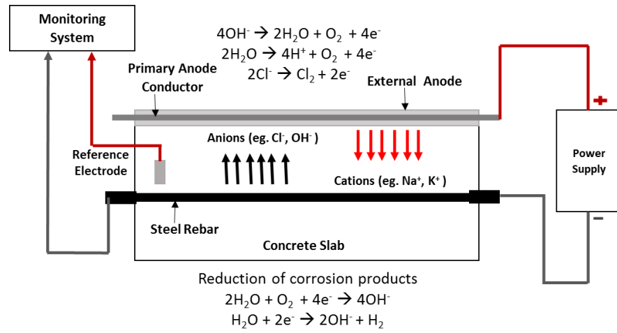
Fig. 11 Schematic of Electrochemical Chloride Removal
