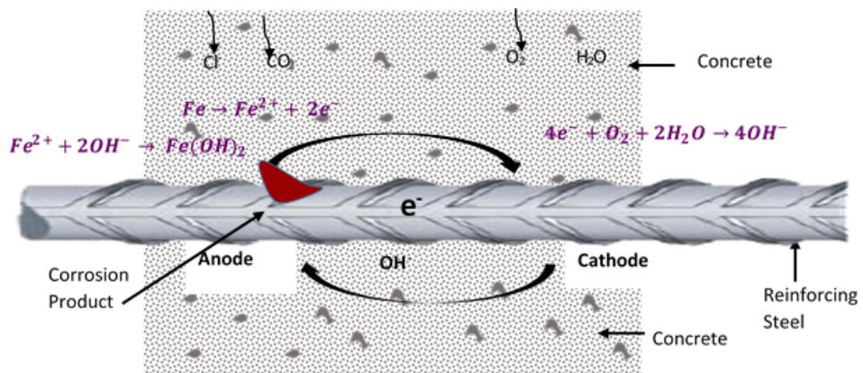
Fig. 1 Schematics of corrosion process in concrete
